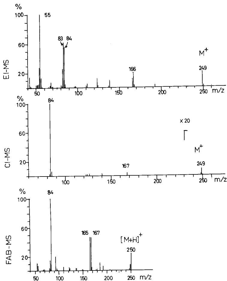
Fig. 3. Mass spectra (EI, CI, FAB-MS) of \alpha -tripiperidine.
