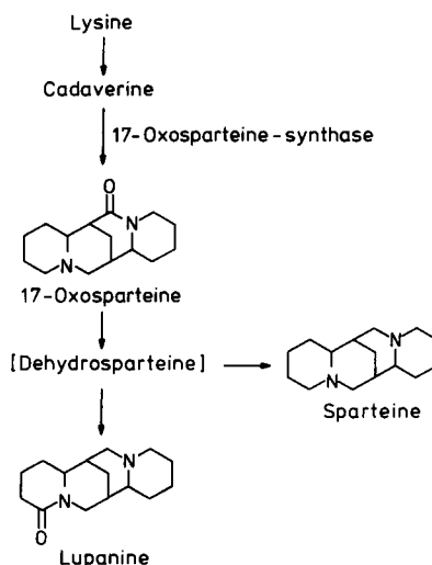
Fig. 1. Possible pathway of lupanine biosynthesis.
